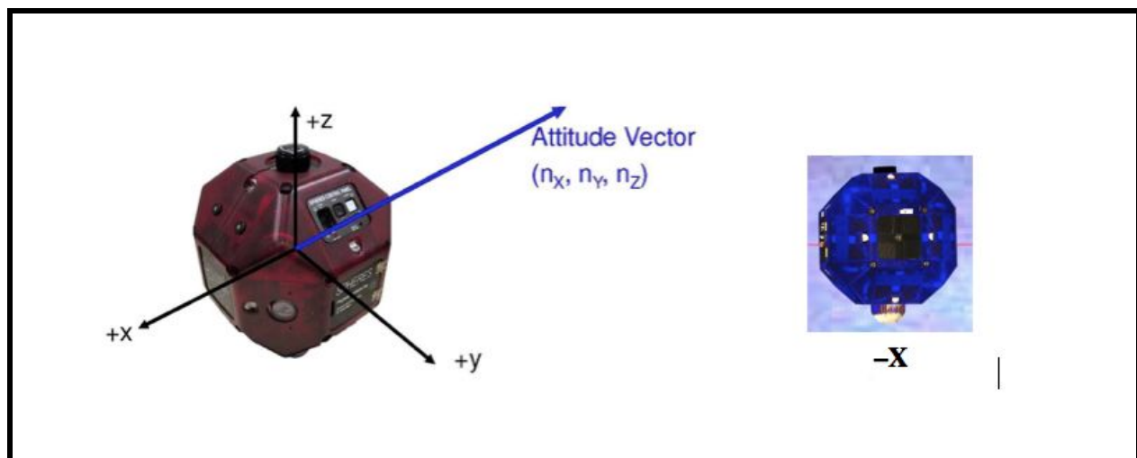
Figure 4: SPHERES points and docks with its -x face
